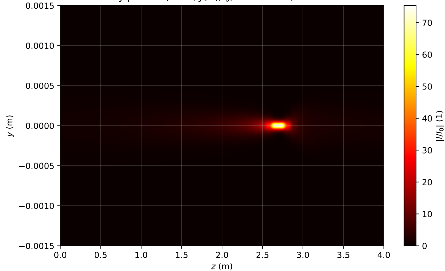
Intensity profile I(x=0, y, z)/I_0 , P_{in}=1.2P_{cr} , artificial time
